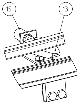
DETAIL B SCALE 1:5
